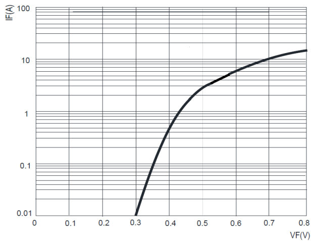
FIG.3: INSTANTANEOUS FORWARD CHARACTERISTICS
