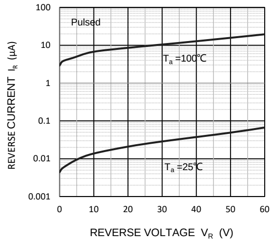
Reverse Characteristics
