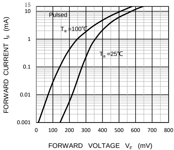
Forward Characteristics
