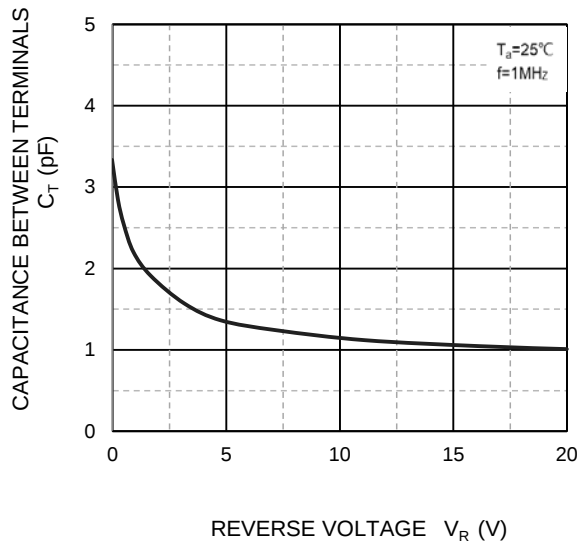
Capacitance Characteristics
