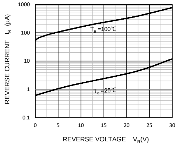
Reverse Characteristics
