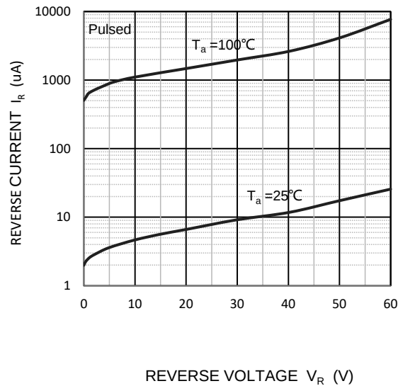
Reverse Characteristics
