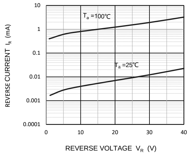
Reverse Characteristics
