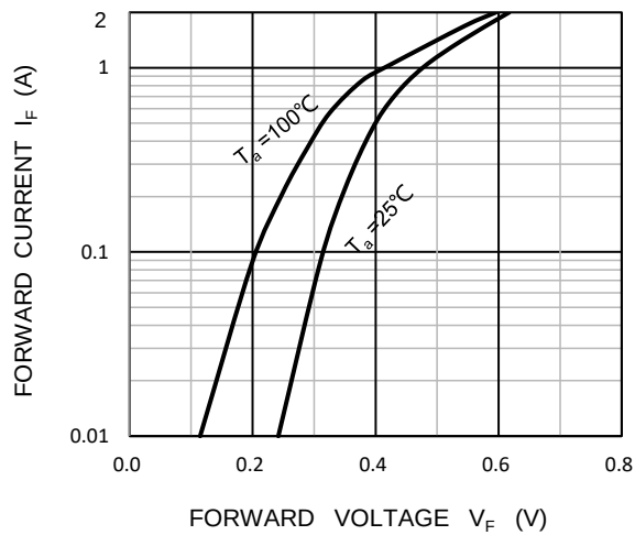
Forward Characteristics
