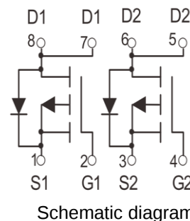
SOP-8 top view
