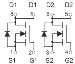
Schematic diagram
