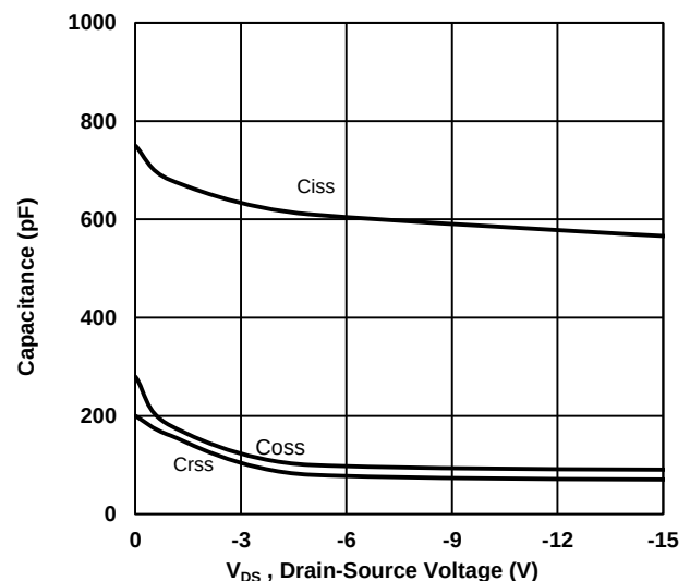
Fig12 Typical Capacitance Vs. Drain-Source Voltage
