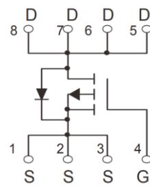
Schematic diagram
