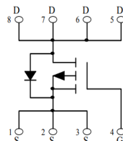
Schematic diagram
