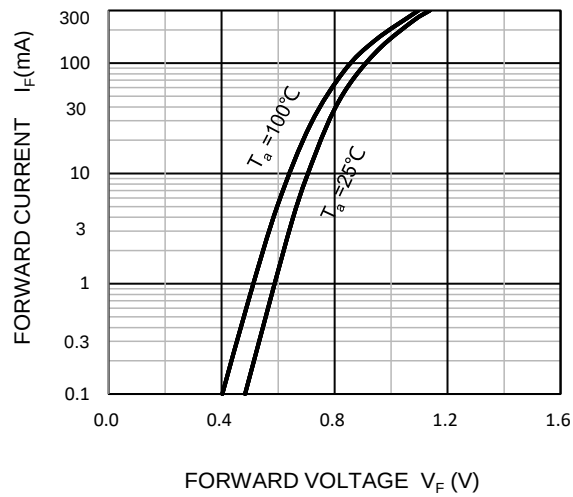
Forward Characteristics
