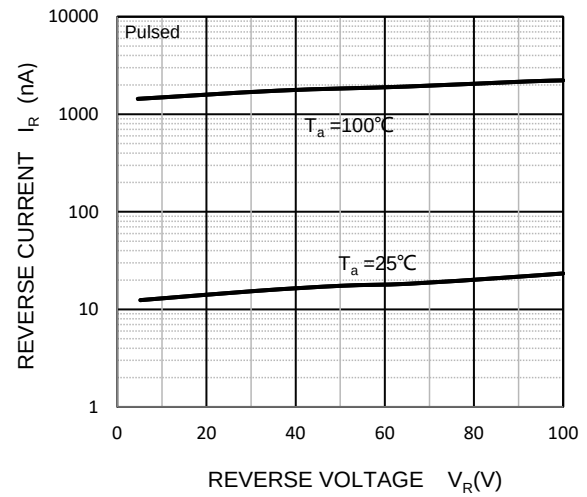
Reverse Characteristics
