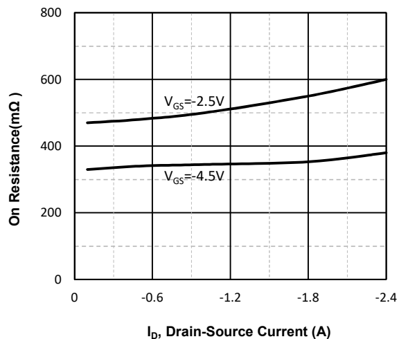
Fig3. On Resistance Vs. Drain-Source Current
