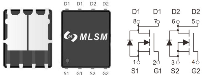
PDFN5X6-8L view
