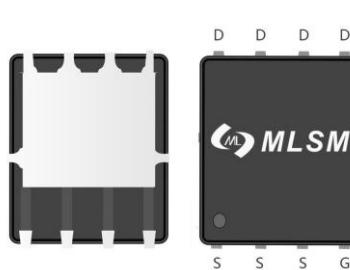
PDFN5X6-8L view
